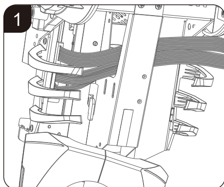
4. Cable the graphics card after it is installed
