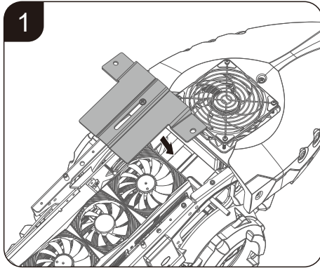
6. GPU assembly process IV
